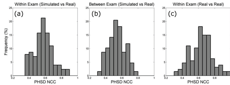
Figure 5.4 Distributions of maximal NCC of pixel standard deviation maps between real and simulated data (a) within examination ( PHSD_w ) averaged over all pair-wise comparisons and (b) between examination ( PHSD_b ). (c) The series average NCC values of all pair-wise pixel standard deviation maps between mean topographies in the same series. Value extremes are interpreted as follows: -1: perfectly negatively correlated, 0: uncorrelated, 1: perfectly positively correlated.
