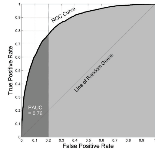
Figure 3.3 Example of ROC curve and the dark grey PAUC within a region of the ROC curve with false positives \leq 0.2 . True positive rate is also known as statistical power .
