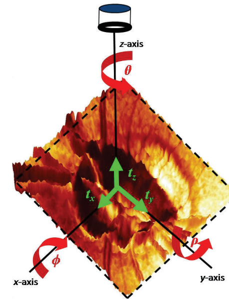
Figure 4.4 Sample HRT Classic topography displayed in three dimensions with reflectance intensity colour mapping. Misalignments due to translations (t_x, t_y, t_z) along and rotations (\phi, \rho, \theta) about the (x, y, z) axes are shown. Measurements and translations in the Z-axis are referred to as axial and those in the xy plane as transverse .
