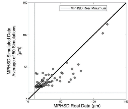
Figure 4.13 MPHSD values for real and simulated mean topographies. The minimum observed MPHSD (10 μm) in real mean topographies is plotted as a lower bound for simulated mean topography MPHSD. Pearson’s sample correlation coefficient r : 0.79 ( p < 0.001 ), MPHSD real – MPHSD simulated mean: 7.6 μm, standard deviation: 13.7 μm.
