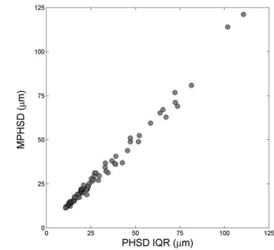
Figure 4.11 MPHSD values compared to inter-quartile range (IQR) values for PHSD distributions.
