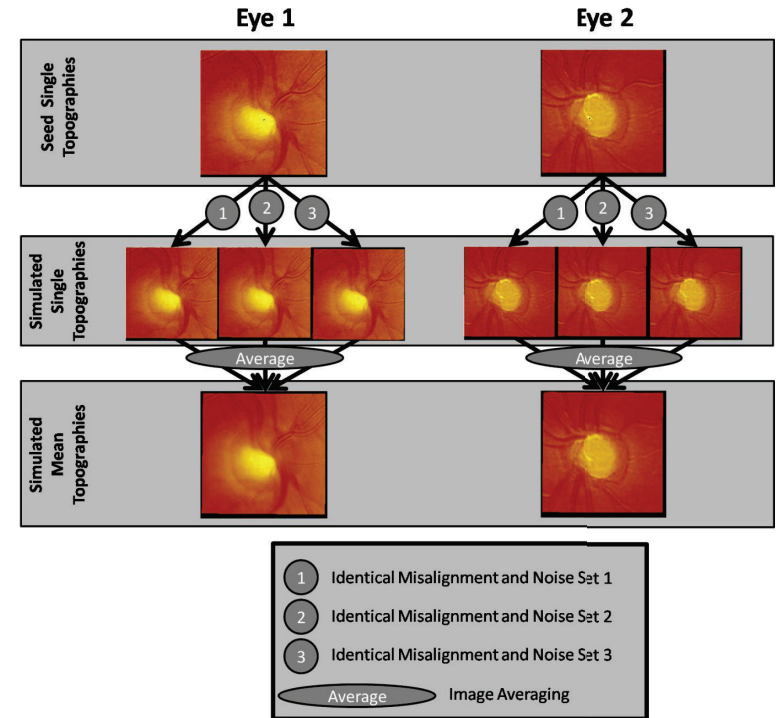
Figure 4.5 The simulation schematic with three different, random misalignment and noise sets applied to a seed single topography to produce three simulated single topographies for two sample eyes. In this example each set applied is identical for both eyes and this is the case across all seed topographies in the analysis.
