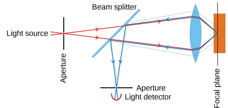
Figure 1.4 Principles of confocal scanning showing the placement of apertures/pinholes in front of the light source/laser and the detector. With an infinitesimally small aperture any light returning from planes posterior or anterior to the focal plane is rejected.
