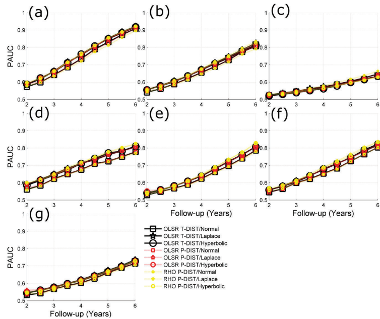
Figure 3.5 Changes with follow-up period of PAUC values (false positive rate < 20%) for the three change detection methods for the three indicated noise distributions in series of a medium trend of RA deterioration ( -0.012\text{mm}^2/\text{year} ). The seven scenarios of noise pattern over time are (a) low uniform noise, (b) medium uniform noise, (c) high uniform noise, (d) medium increasing noise, (e) medium decreasing noise, (f) medium noise with an outlier measurement and (g) medium noise with autocorrelation. See Figure 3.2 for illustration of noise patterns.
