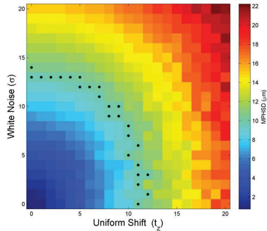
Figure 4.6 The relationship of MPHSD of a 256 x 256 ‘flat’ image with different levels of morphologically independent noise added. Boundary points where MPHSD values are produced corresponding with the minimum MPHSD observed in real data (10μm) are indicated.
