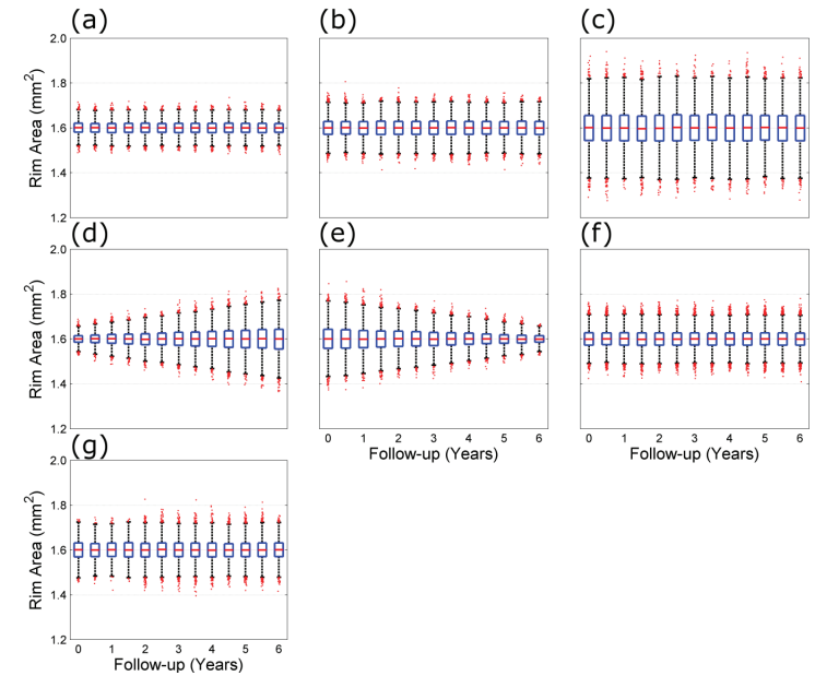
Figure 3.2 Box-whisker plots showing the spread of normally distributed measurement variability at each follow-up examination for stable series. Each panel represents a scenario of measurement variability with the following average magnitudes and its change across the follow-up period: (a) uniform low noise, (b) uniform medium noise, (c) uniform high noise, (d) medium increasing noise, (e) medium decreasing noise, (f) medium noise with an outlier present, and (g) medium noise with autocorrelation.
