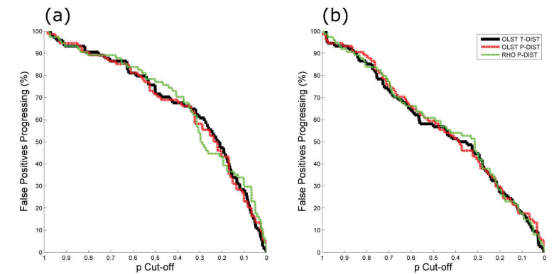
Figure 3.4 (a) HRT Classic data: Percentage of falsely flagged progressing series at fifth and final examination for the p-value cut-off of each change detection test (b) HRT II data: Percentage of falsely flagged progressing series at fifth and final examination for the p-value cut-off of each change detection test.
