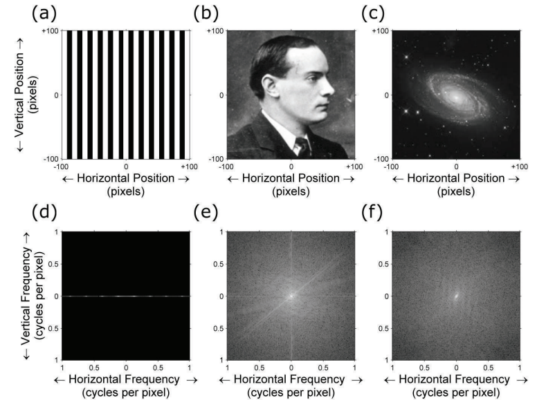
Figure 4.7 Fourier analysis example of (a) an image with periodic vertical stripes, (b) photograph of Pádraig Mac Piarais in side profile, (c) telescope image of the M91 galaxy, (d) power spectrum of (a), (e) power spectrum of (b), (f) power spectrum of (c). The brighter the points in (d), (e) and (f) indicate the higher amplitude of a given frequency - lower frequencies are located towards the centre of these images and higher frequencies towards the edges. Note that log scales for the intensity are used for (d), (e) and (f) as the proportions of frequency components at the centre (representing the average of the signal) and at key characteristic frequencies are much higher than elsewhere.
